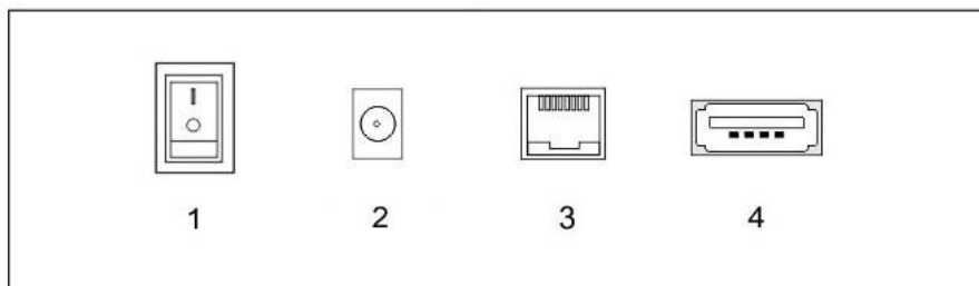
1. ON/OFF Switch 2. Power Port 3. RJ45 (Ethernet) 4. USB port
